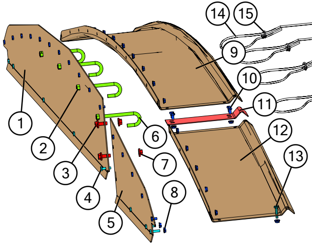
Rear Endcap
